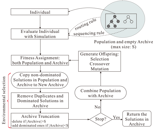
Fig. 4. Overview of SPMTGP2.
